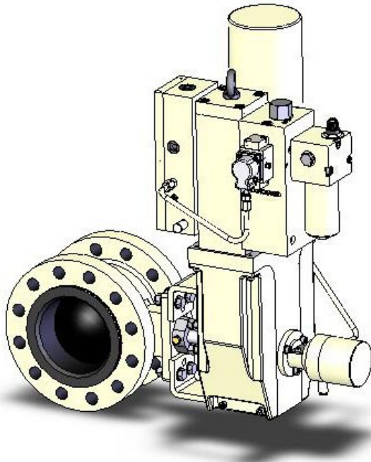
The Fuel Gas Stop Ratio Control system on Frame 7FA gas turbines.
